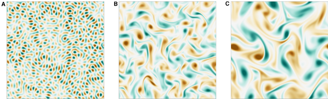
Fig. 1 Evolution of a decaying turbulent 2D flow at initial time (A), intermediate time (B), end time of the simulation (C). The colours represent the vorticity field.
